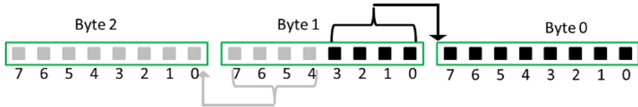
Figure 1. Packing two 12-bit pixels into three bytes.
