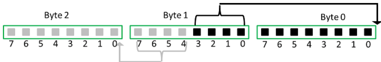
Figure 2. Packing two 12-bit pixels into three bytes.
